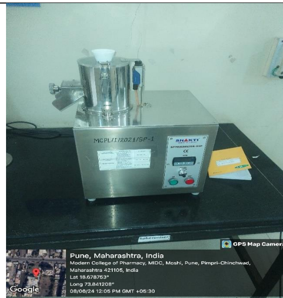
Spheronizer
