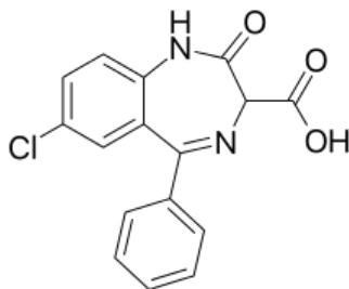
Clorazepate
