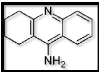
Fig. Tacrine
